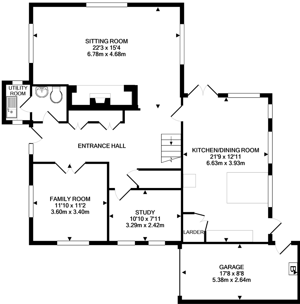
GROUND FLOOR APPROX. FLOOR AREA 1228 SQ.FT. (114.1 SQ.M.)
