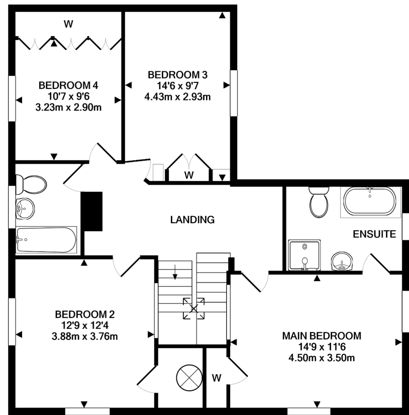
1ST FLOOR APPROX. FLOOR AREA 935 SQ.FT. (86.9 SQ.M.)
